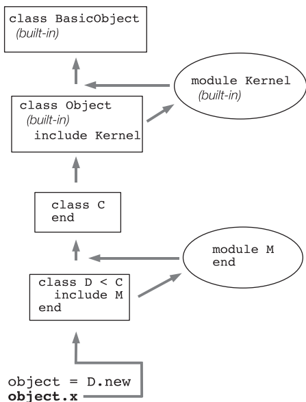
Figure 4.1 An instance of class D looks for method x in its method search path.
