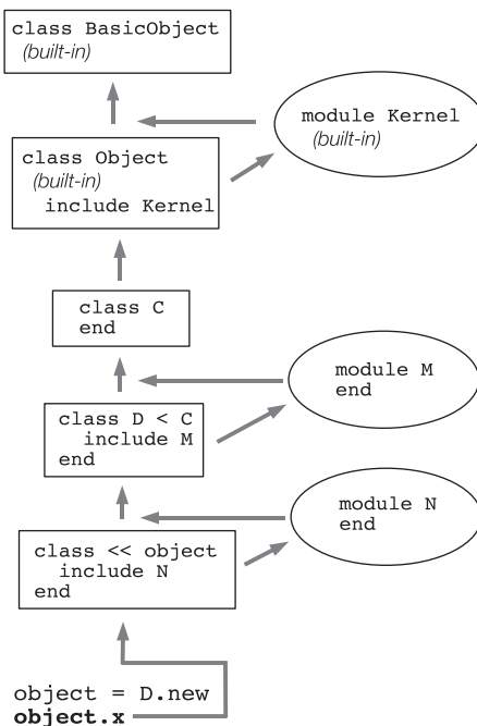
Figure 13.1 Method-search order, revised to include singleton classes
