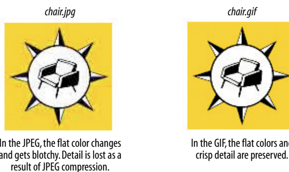
Figure 22-11. The same flat graphical image saved as both a JPEG and a GIF.
