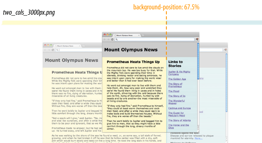
Figure 16-19. The background image is anchored at the point between the two columns, so when the browser window gets larger or smaller, it is always in the right place. The graphic file is wide enough that there will be enough image to fill both columns, even on the widest of browsers.
