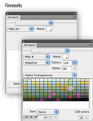
Figure 22-16. PNG-24 and PNG-8 settings in Photoshop and Fireworks.
