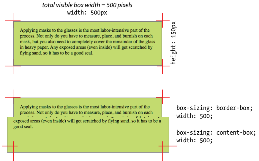
Figure 14-3. Sizing an element with the border-box method. The bottom diagram compares the resulting boxes from each sizing method.
