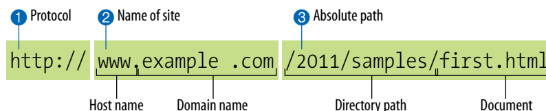
Figure 2-1. The parts of a URL.
