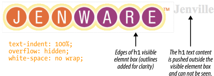
Figure 18-1. The Kellum image replacement technique hides the HTML text by pushing it out of the visible element box with a text indent.
