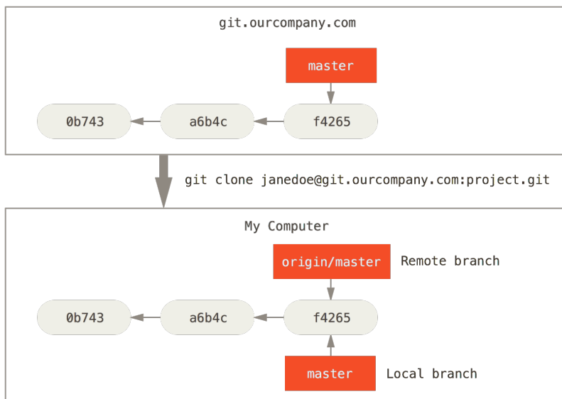
FIGURE 3-22 Server and local repositories after cloning
