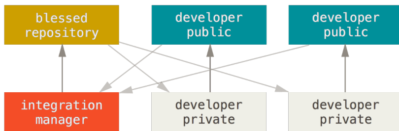
FIGURE 5-2 Integration- manager workflow.
